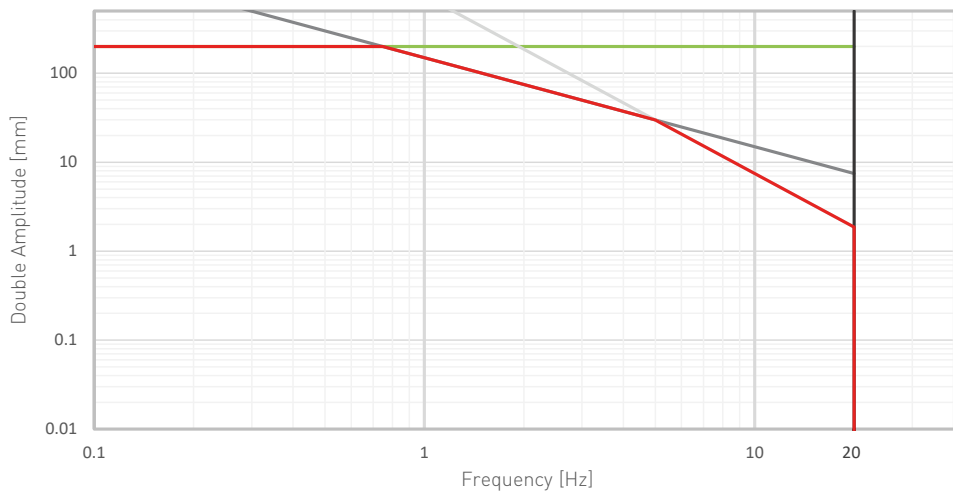
Performance chart - EA050-7F/40/24A-B20/1.41-200
