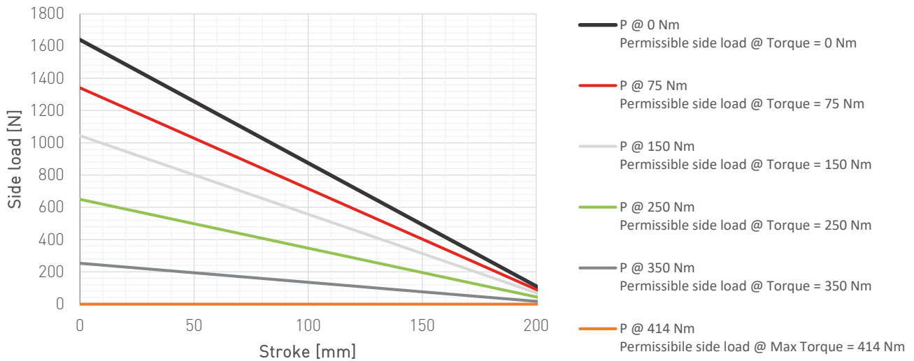
Permissible side load for a given torque EA100 - stroke 200 mm
