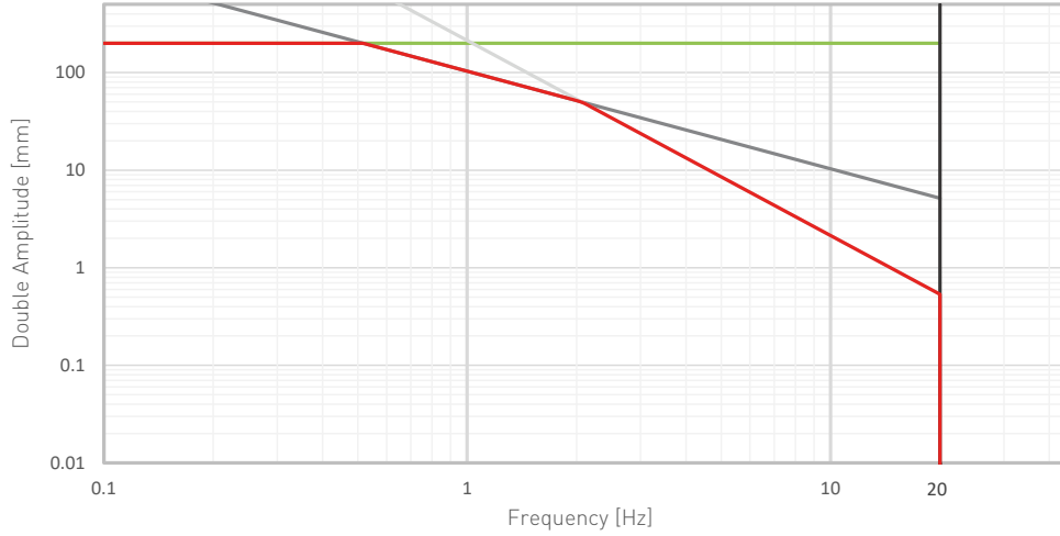
Performance chart - EA050-5/12/6A-N10/1.55-200
