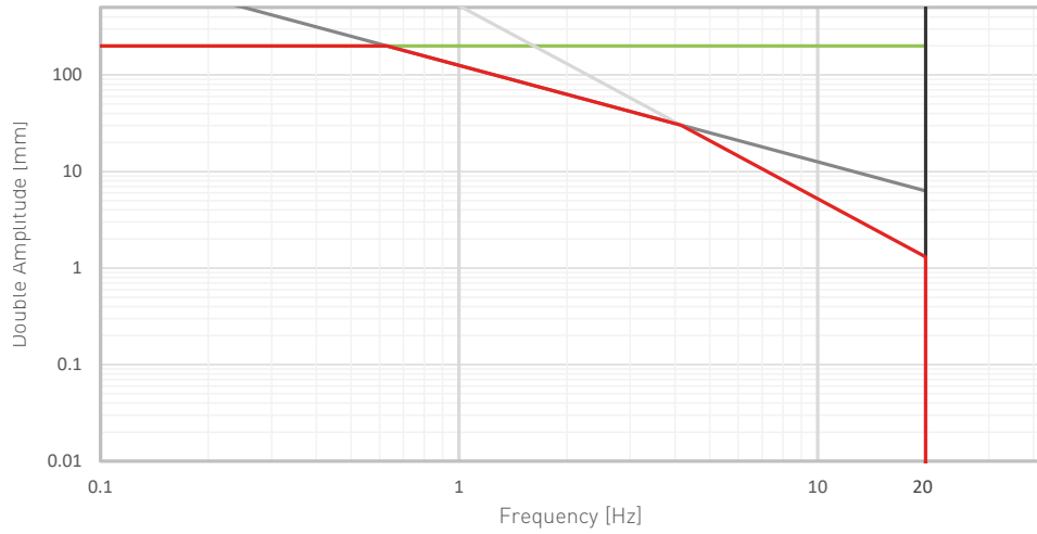
Performance chart - EA050-7/40/12A-B20/1.69-200
