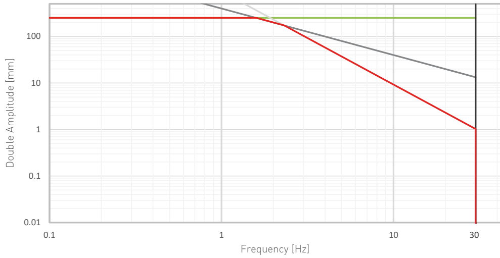
Performance chart - EA05-3/04/3A-T25/1-250
